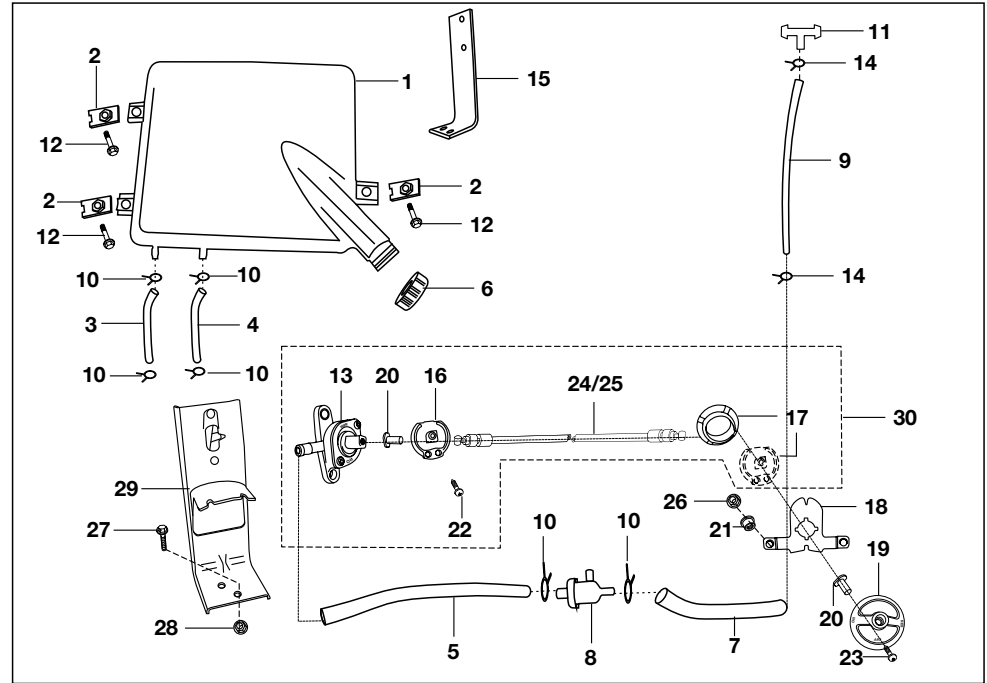
Plate No. 30 : PETROL TANK & PETROL COCK ASSLY
